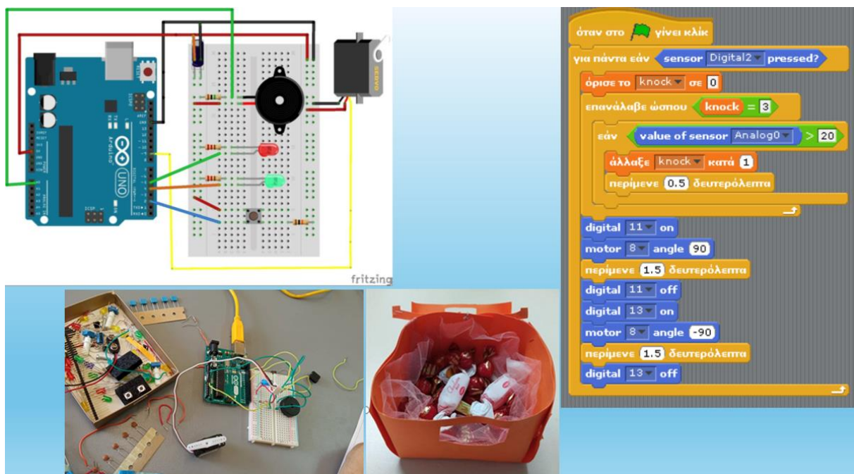
Figure 3. The circuit in Tinkercad, the real circuit during construction, the program and the treasure chest.
