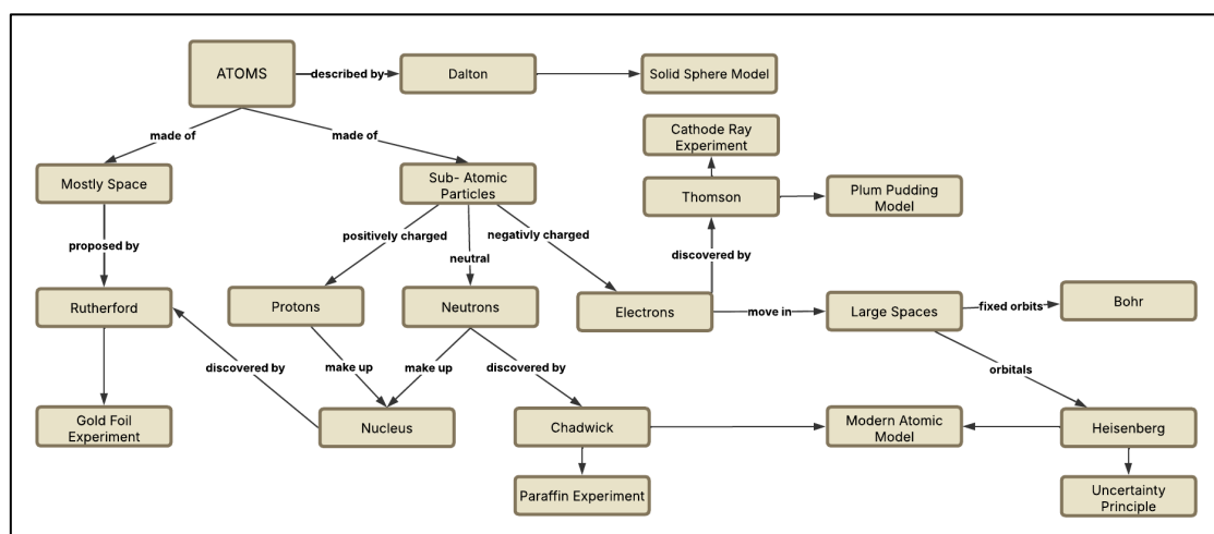
Figure 1. Concept map related to atomic models.
