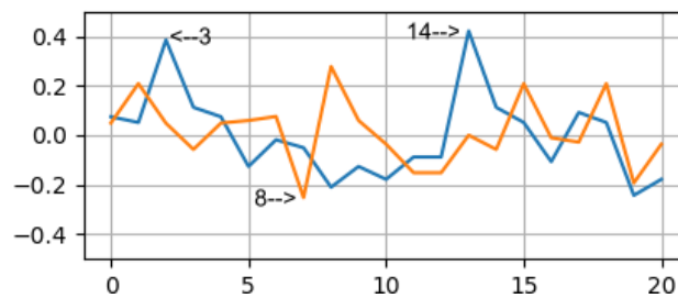
Figure 5. Stable pattern \vec{U}_{11} of relations.
