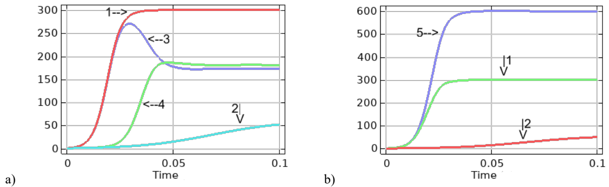
Figure 4. Simulation of evolution of predator-prey system (a) and prey-prey cooperation (b). 1,2 – separated prey and predator respectively; 4,3 – predator-prey system; 5 - prey-prey cooperation
