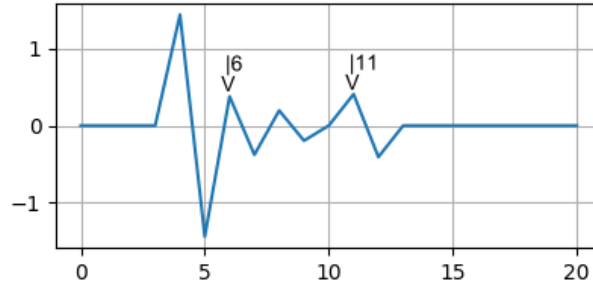
Figure 2. Imaginary part of eigenvalues spectrum of interaction matrix.
