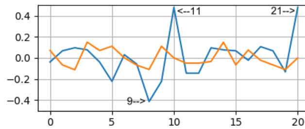
Figure 3. Stable scheme \vec{U}_6 of relations.
